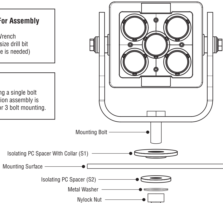
Isolation Assembly Diagram:
