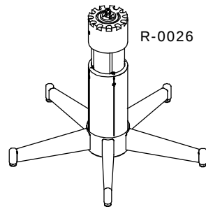
Spare Column and Base for: 6530 NS1500 Office Comfort Sitting height:690/850
