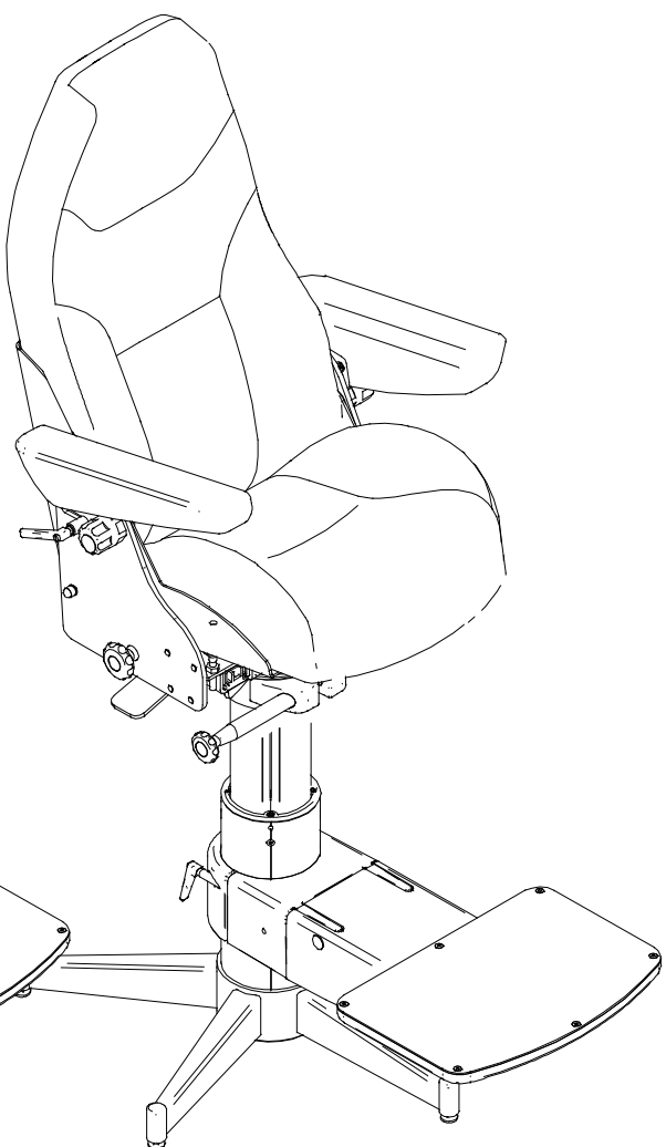
COMFORT 6525 h=850/1070 6530 h=690/850 6535 h=630/730
