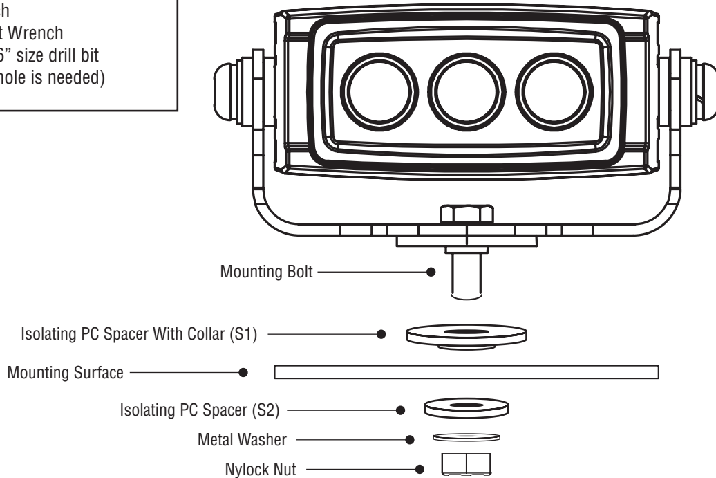
Isolation Assembly Diagram:
