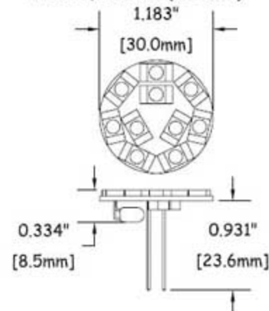
X-Beam, Back Pin (G4/GU4)
