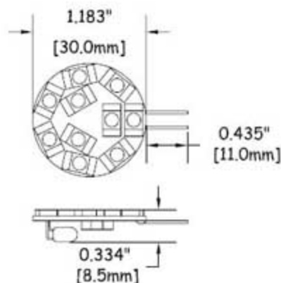
Novi (Blue), Side Pin (G4)
