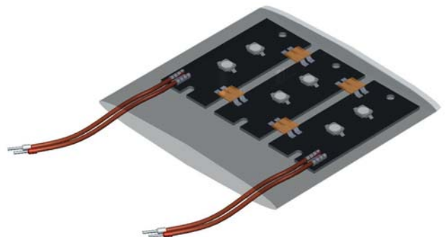
LED MC-PCB
