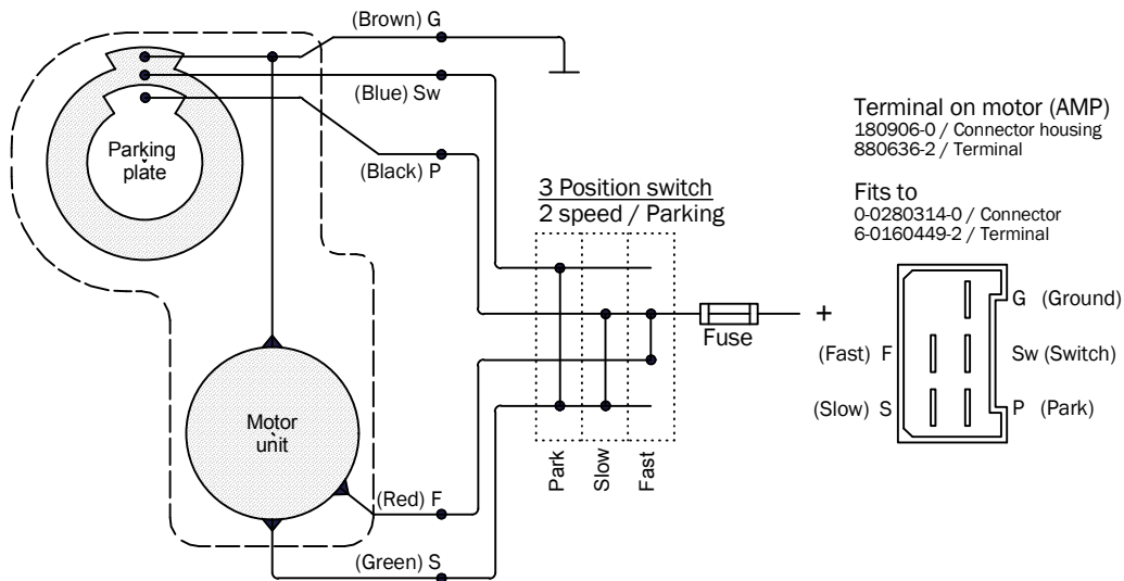
Alt. 1 (3 pos.switch)
